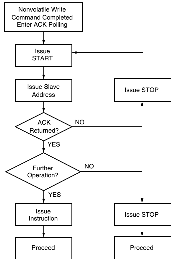
Flow 1. ACK Polling Sequence
