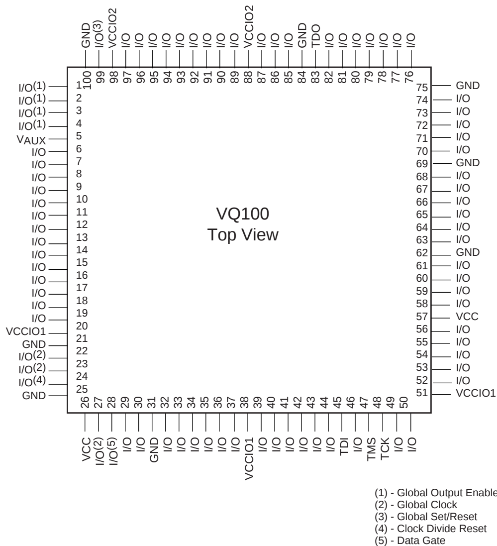
Figure 6: VQ100 Very Thin Quad Flat Pack
