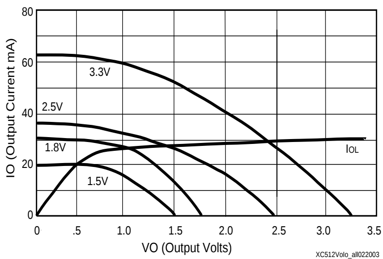
Figure 4: Typical Derating Curve for XC2C512
