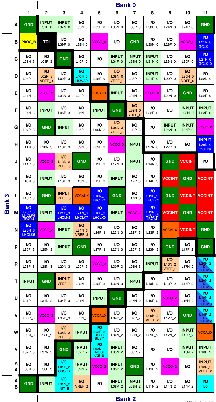
Figure 89: FG484 Package Footprint (top view)
