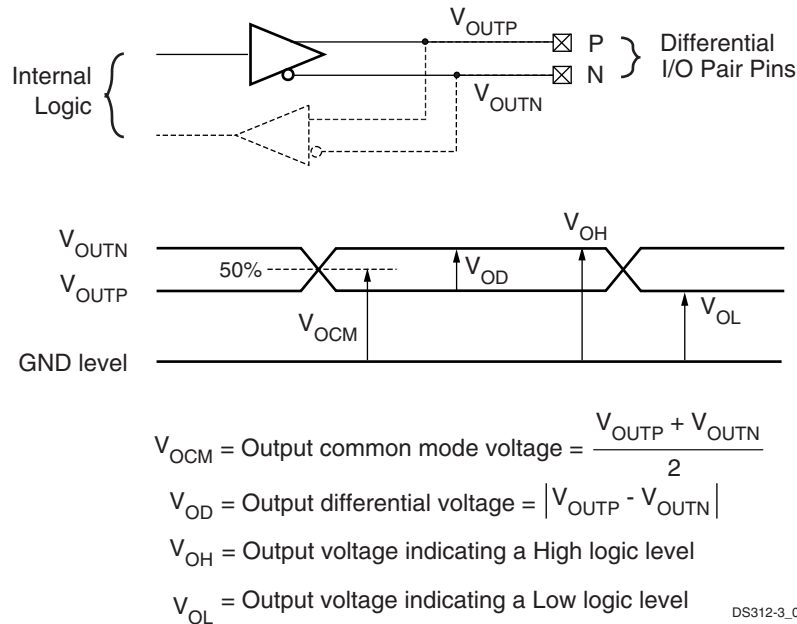
Figure 71: Differential Output Voltages
