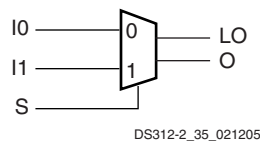
Figure 21: F5MUX with Local and General Outputs
