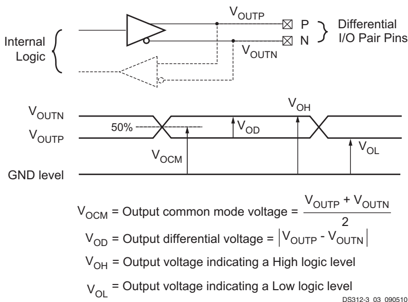
Figure 4: Differential Output Voltages
