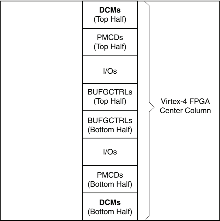
Figure 2-1: DCM Location
