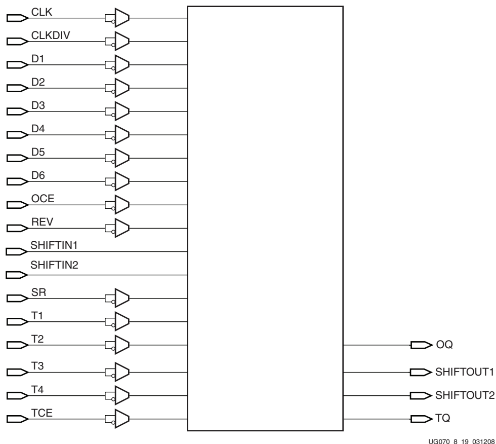
Figure 8-15: OSERDES Primitive
