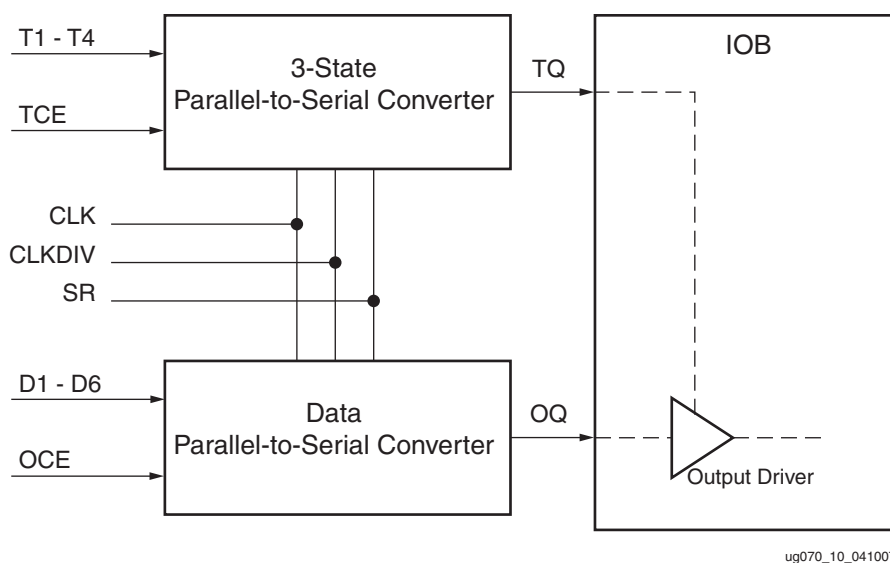
Figure 8-14: OSERDES Block Diagram
