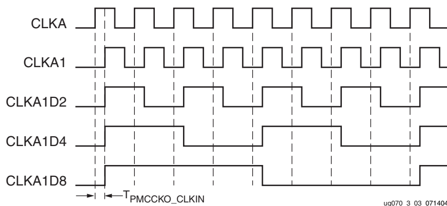
Figure 3-3: PMCD Frequency Divider
