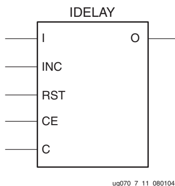
Figure 7-11: IDELAY Primitive
