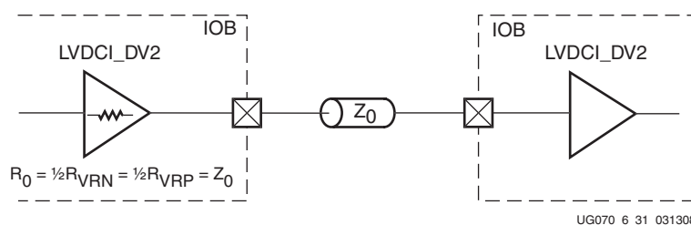
Figure 6-31: Controlled Impedance Driver with Half Impedance Unidirectional Termination
