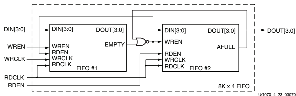
Figure 4-22: Cascading FIFO
