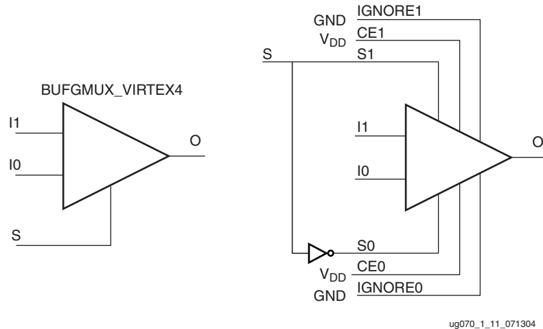
Figure 1-11: BUFGMUX_VIRTEX4 as BUFGCTRL
