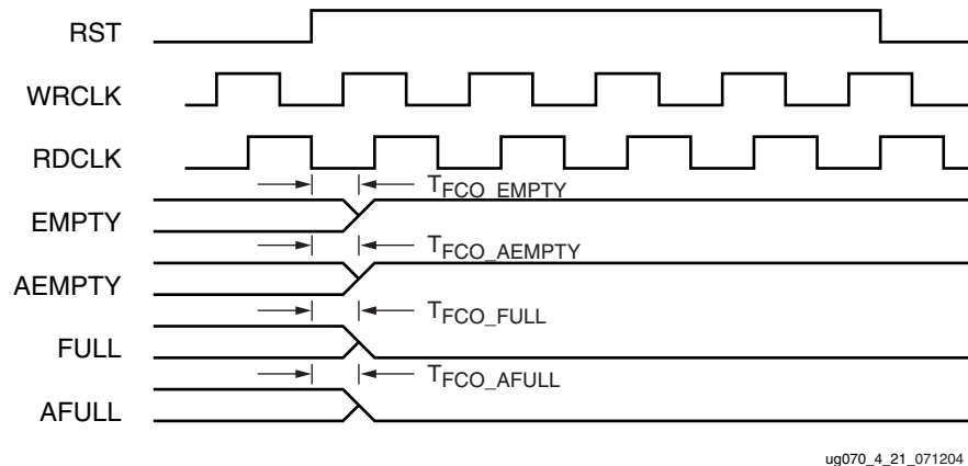
Figure 4-21: Resetting All Flags
