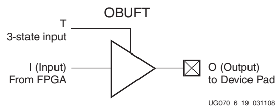
Figure 6-19: 3-State Output Buffer (OBUFT) Primitive
