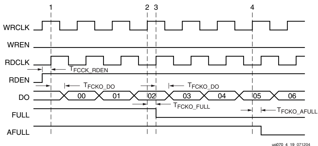
Figure 4-19: Reading From a Full FIFO
