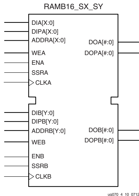
Figure 4-10: Dual-Port Block RAM Primitive
