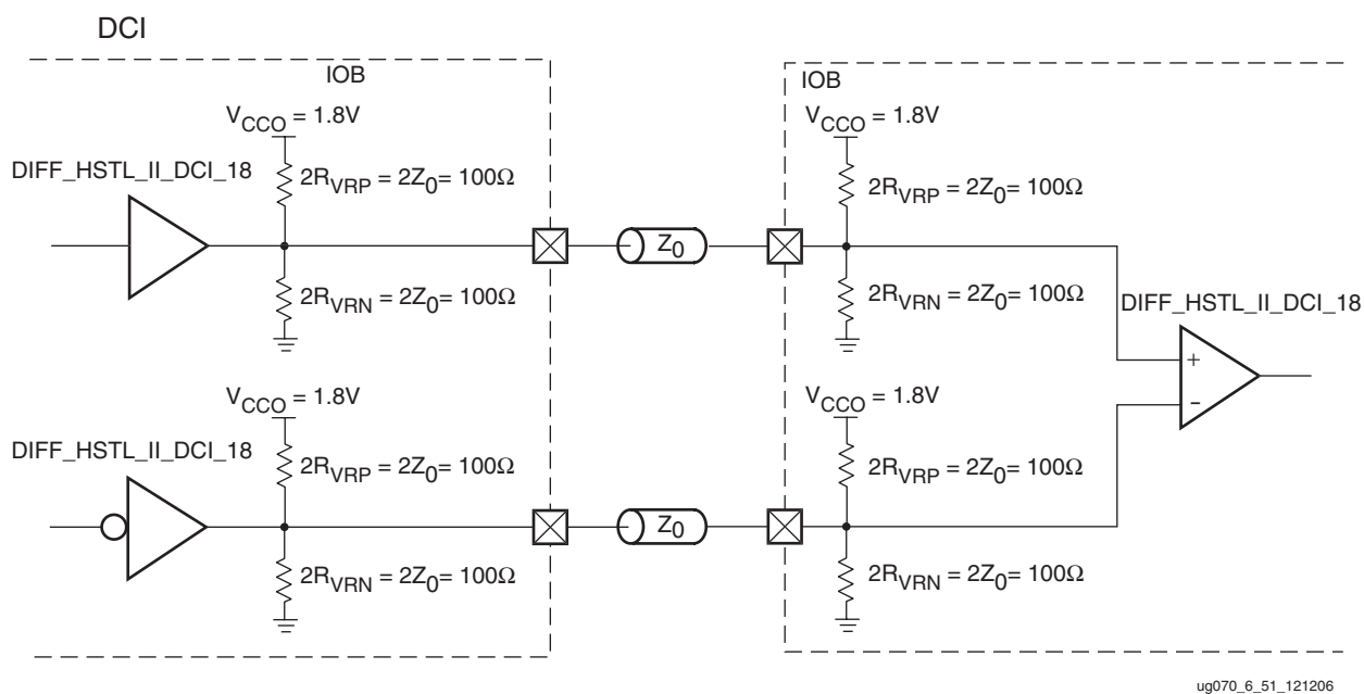
Figure 6-53: Differential HSTL (1.8V) Class II DCI Unidirectional Termination
