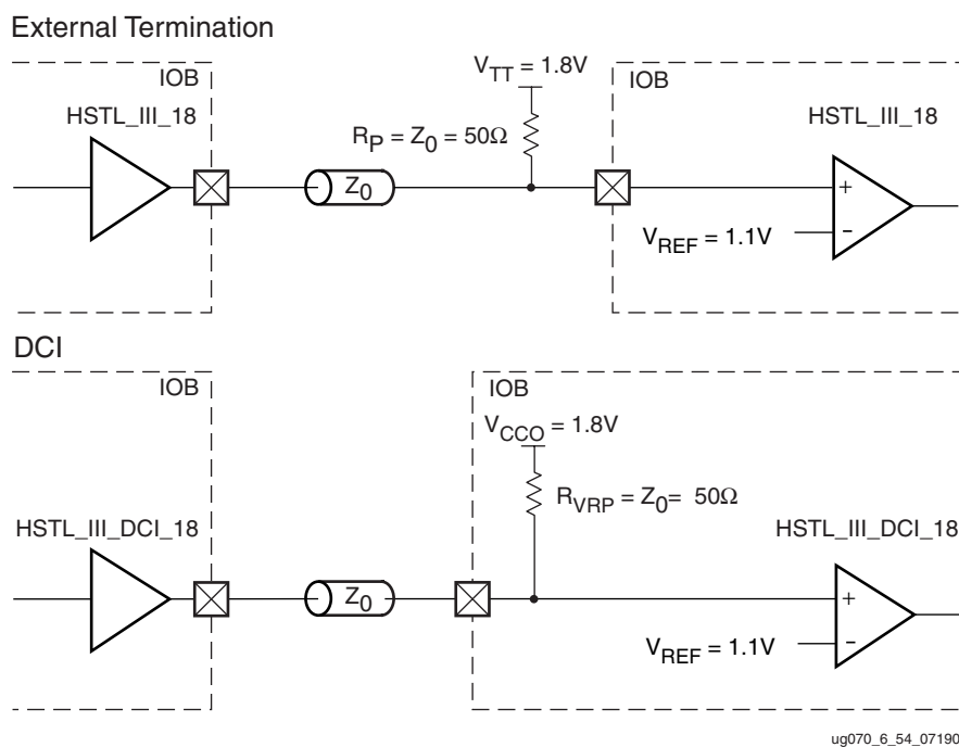
Figure 6-56: HSTL Class III (1.8V) Termination
