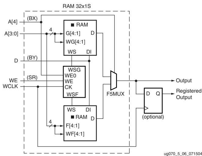
Figure 5-6: Single-Port Distributed RAM (RAM32x1S)
