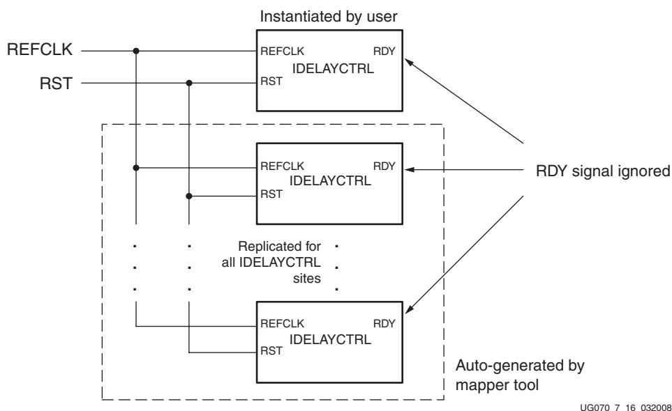
Figure 7-16: Instantiate IDELAYCTRL without LOC Constraints - RDY Unconnected
