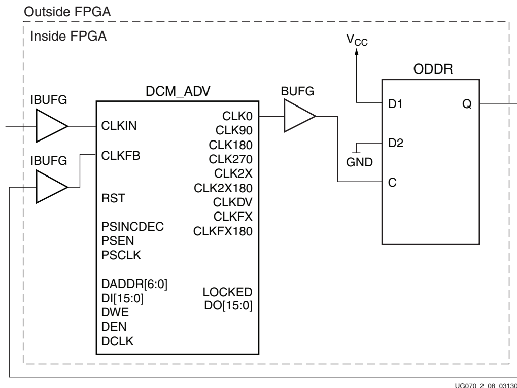
Figure 2-9: Board-Level Clock Using DDR Register with External Feedback
