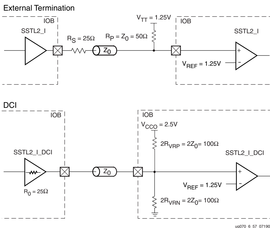
Figure 6-59: SSTL2 Class I Termination
