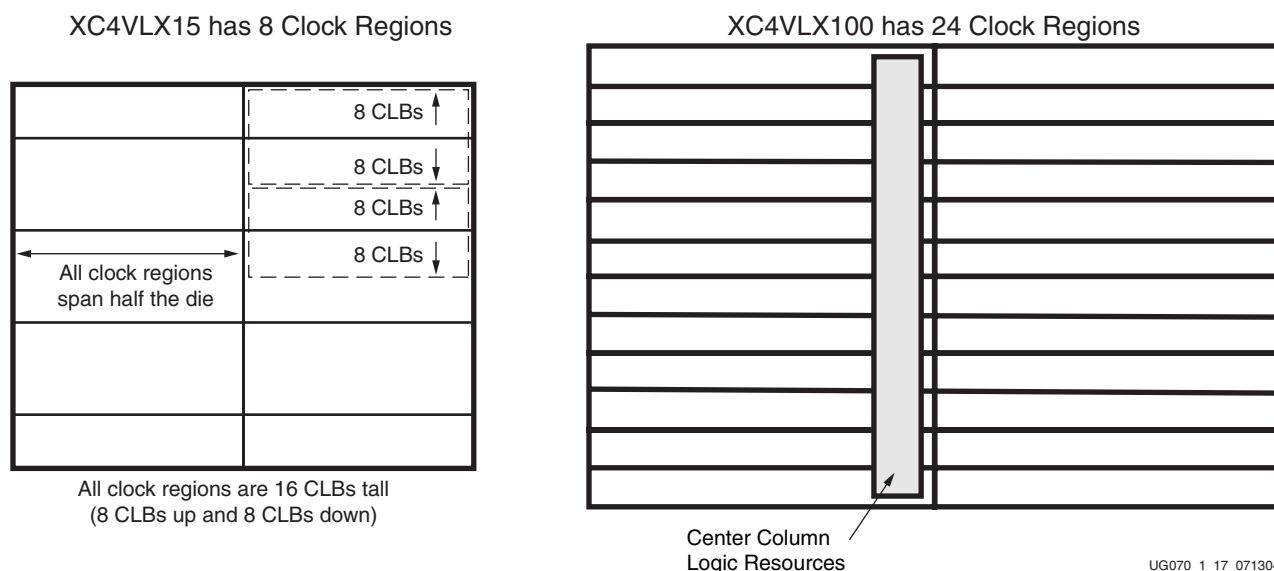
Figure 1-17: Clock Regions
