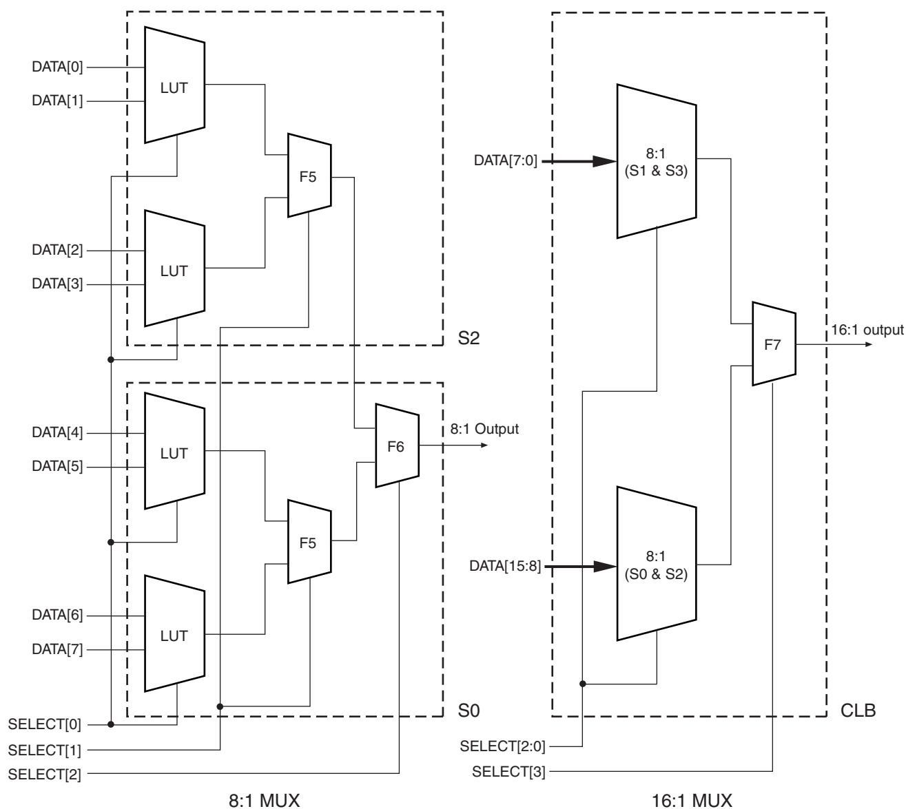
Figure 5-18: 8:1 and 16:1 Multiplexers
