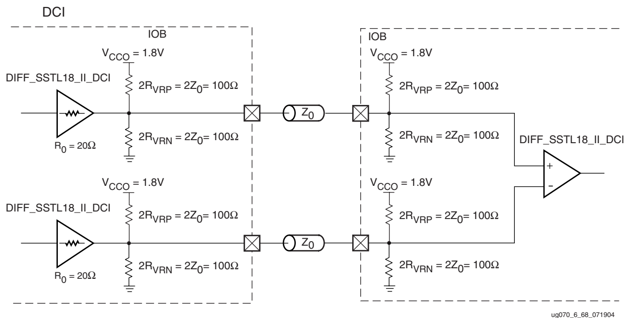
Figure 6-70: Differential SSTL (1.8V) Class II Unidirectional DCI Termination
