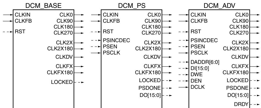
Figure 2-2: DCM Primitives
