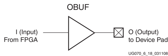
Figure 6-18: Output Buffer (OBUF) Primitive
