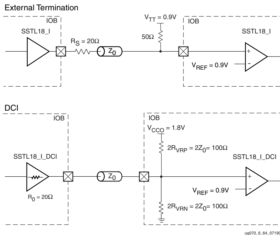
Figure 6-66: SSTL18 (1.8V) Class I Termination
