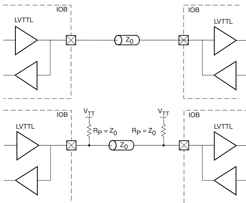
Figure 6-26: LVTTL Bidirectional Termination
