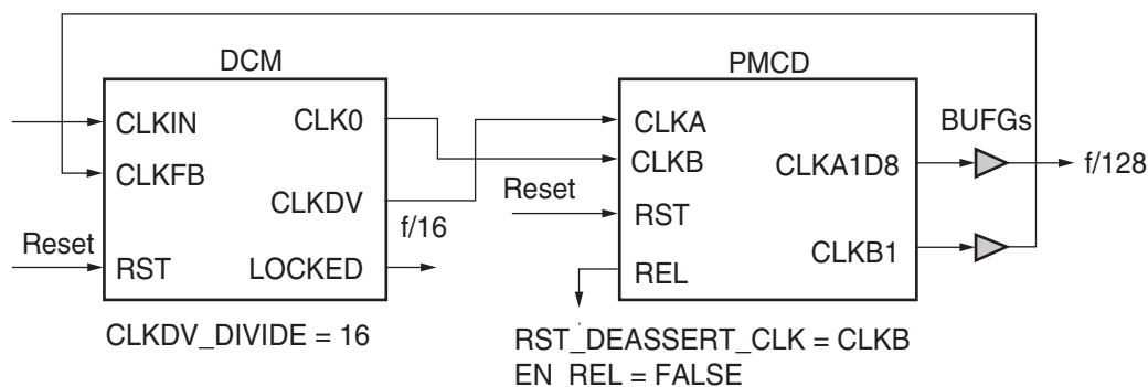
Figure 3-11: DCM to PMCD for Clock Frequency Division
