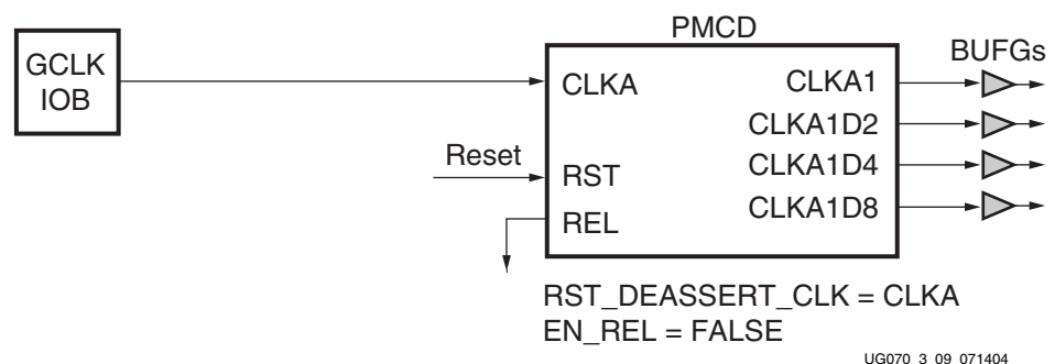
Figure 3-9: PMCD Driven by IBUFG (GCLK IOB)
