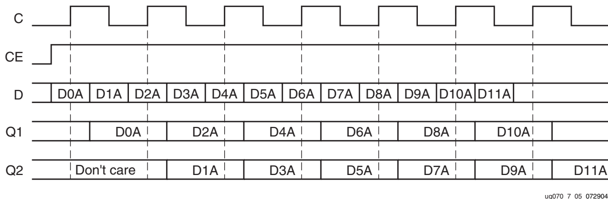
Figure 7-5: Input DDR Timing in SAME_EDGE Mode
