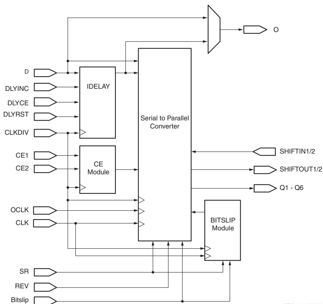
Figure 8-1: ISERDES Block Diagram
