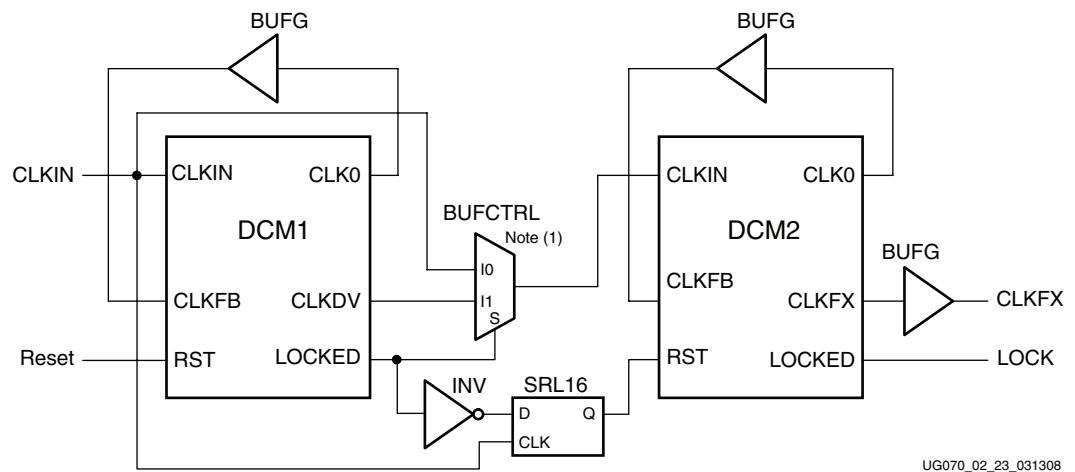
Figure 2-5: Cascading DCMs
