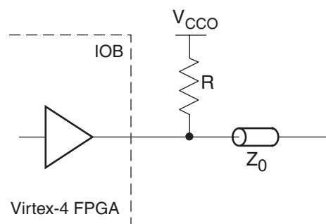
Figure 6-10: Driver with Termination to V_{CCO} without DCI
