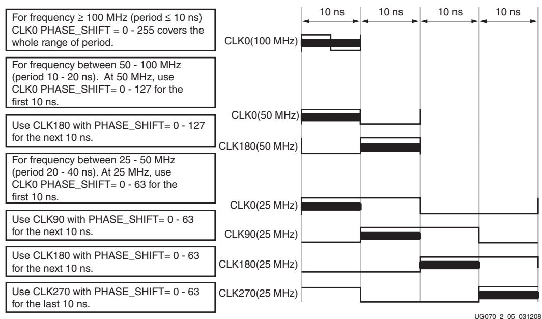
Figure 2-6: Fixed Phase-Shift Examples
