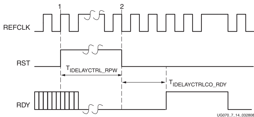
Figure 7-14: Timing Relationship Between RST and RDY
