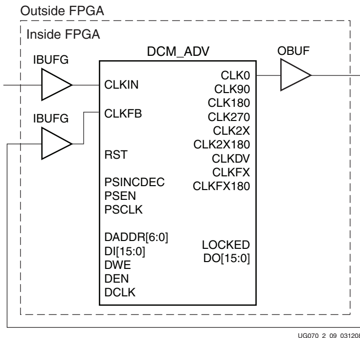
Figure 2-10: Board-Level Clock Using OBUF with External Feedback
