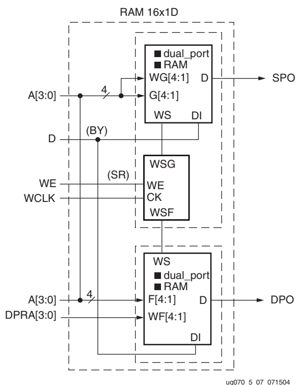
Figure 5-7: Dual-Port Distributed RAM (RAM16x1D)
