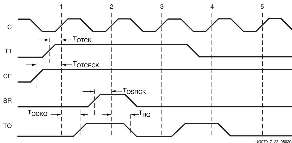
Figure 7-28: OLOGIC 3-State Register Timing Characteristics
