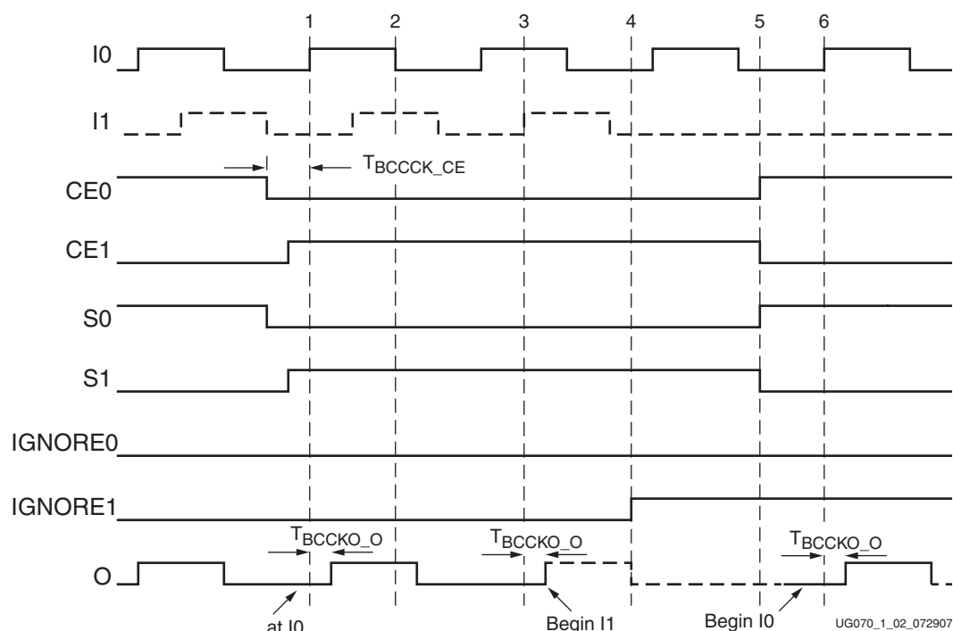
Figure 1-2: BUFGCTRL Timing Diagram
