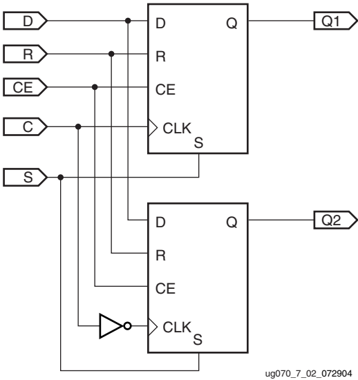
Figure 7-2: Input DDR in OPPOSITE_EDGE Mode
