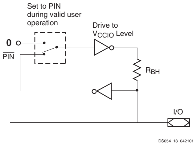
Figure 13: Bus-Hold Logic
