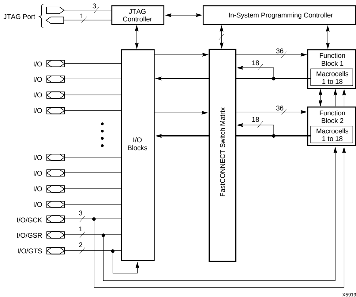
Figure 2: XC9536 Architecture
