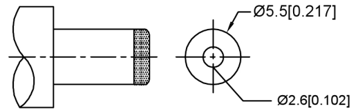
MATING PLUG Jack Insertion Depth: 9.0 mm
