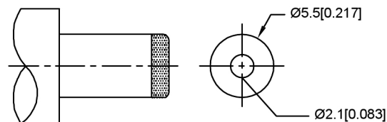
MATING PLUG Jack Insertion Depth: 9.0 mm
