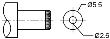
MATING PLUG Jack Insertion Depth: 9.0 mm
