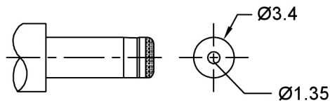
MATING PLUG
