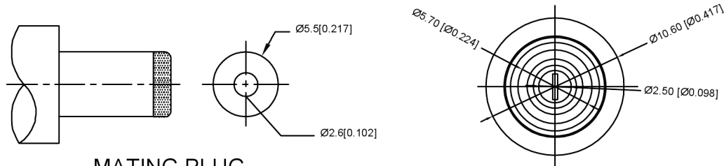
MATING PLUG Jack Insertion Depth: 9.0 mm
