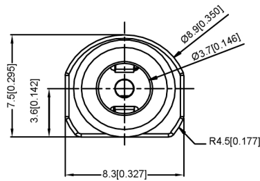
( Ø3.5mm DC PLUG DETAIL DRWING )
