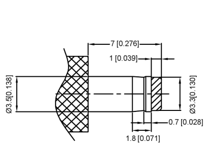
( Ø3.5mm DC PLUG DETAIL DRWING )
