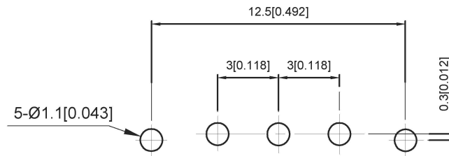
PCB LAYOUT
