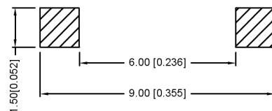
PCB.WELDING DRAWING
