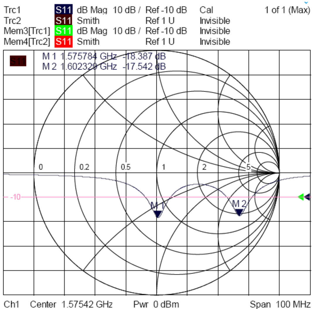
Fig. 3 Return loss
