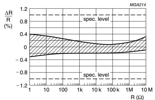
Fig. 17 Typical percentage change in resistance after soldering for 10 seconds at 270 °C, completely immersed
