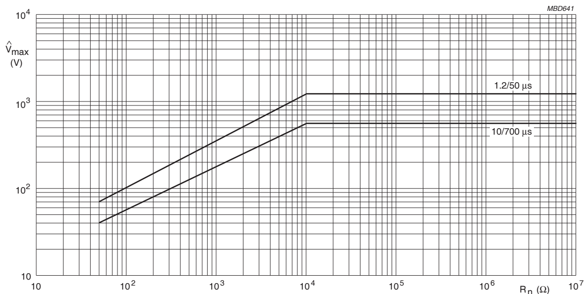
Fig. 11 Maximum permissible peak pulse voltage ( \hat{V}_{max} ) without failing to 'open circuit' in accordance with DIN IEC 60040 (CO) 533
