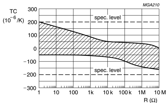
Fig. 16 Typical temperature coefficients between the lower and upper category temperatures
