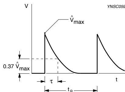
Fig. 15 Exponential pulses
