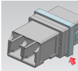
LC EMI Adapter with EMI gasket
