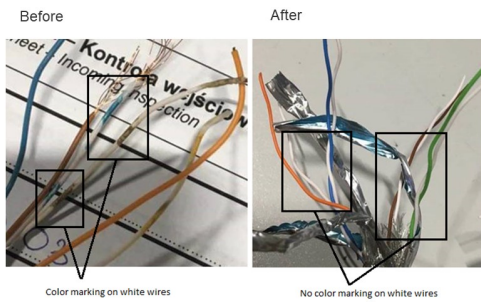
Color marking on white wires
