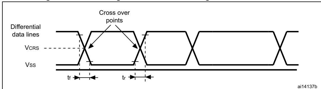
Figure 54. USB timings - definition of data signal rise and fall time
