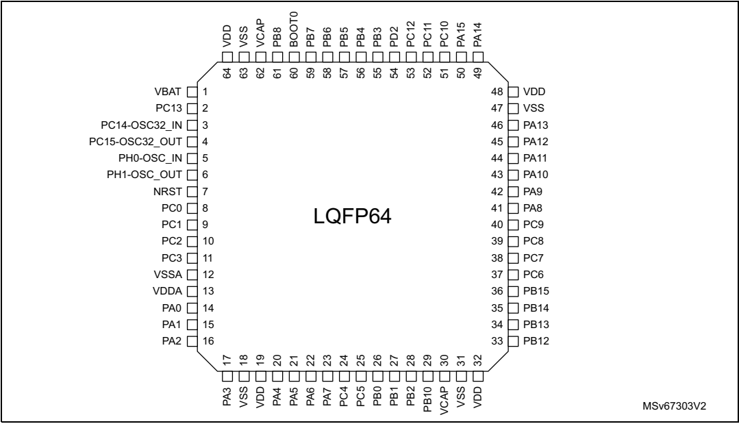
Figure 7. LQFP64 pinout
