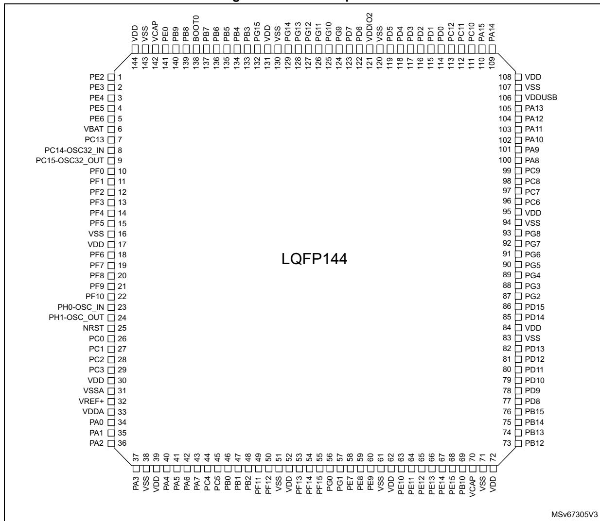
Figure 10. LQFP144 pinout
