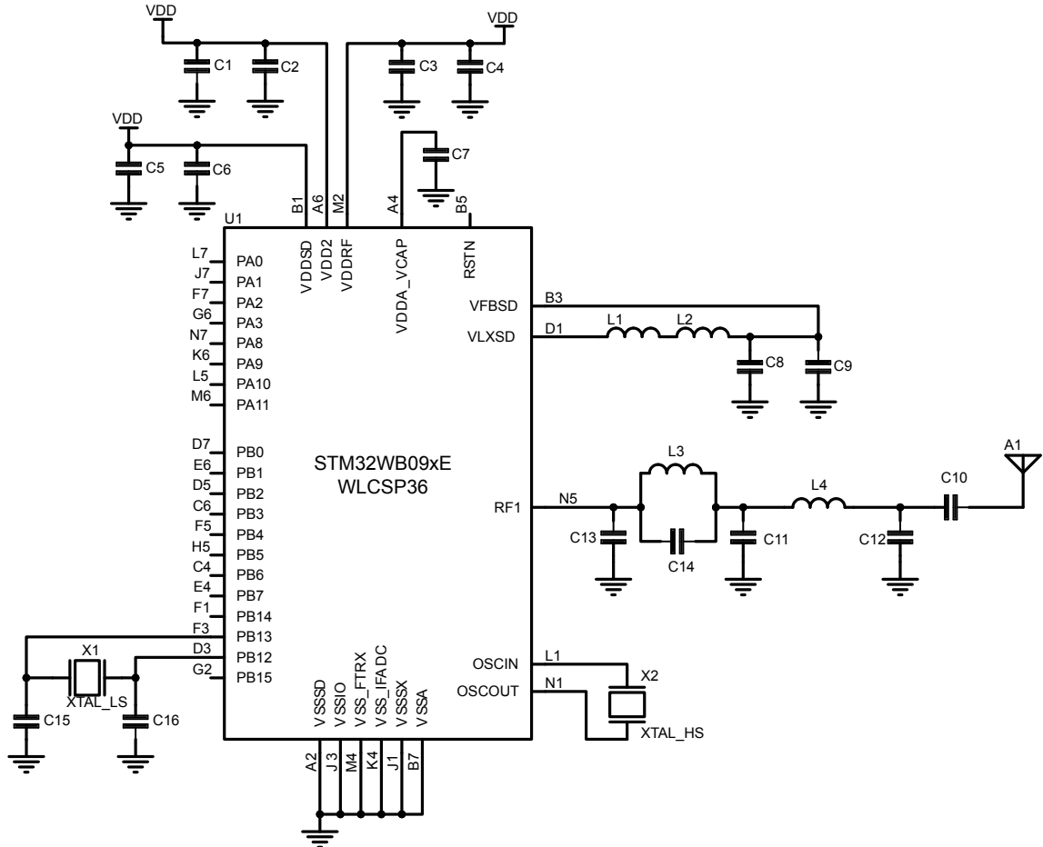
Figure 9. Application circuit: DC-DC converter, WLCSP36 package
