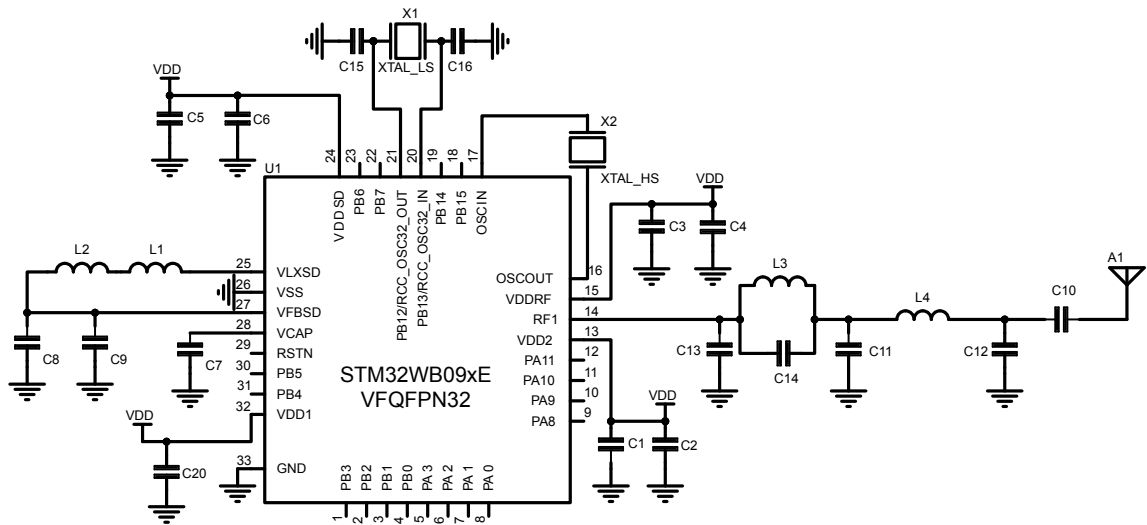
Figure 10. Application circuit: DC-DC converter, VFQFPN32 package
