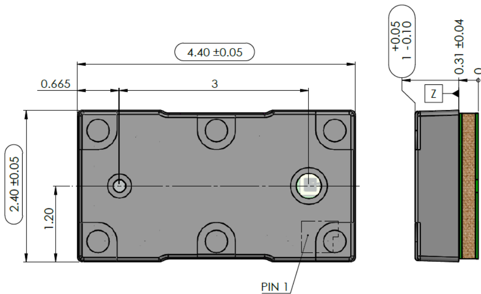
Figure 23. Outline drawing (2/5)
