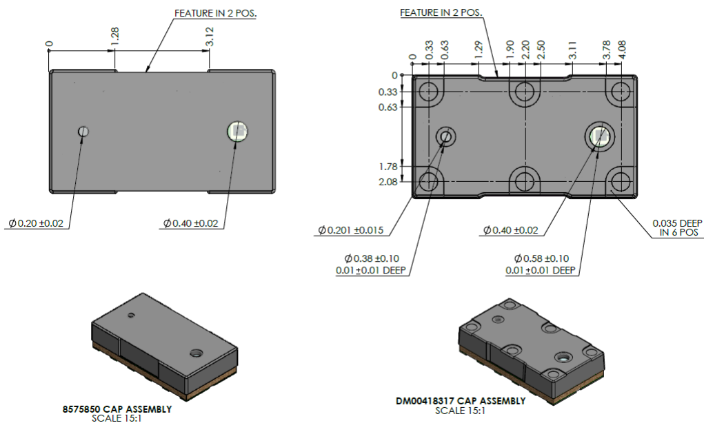
Figure 23. Outline drawing (2/5)
