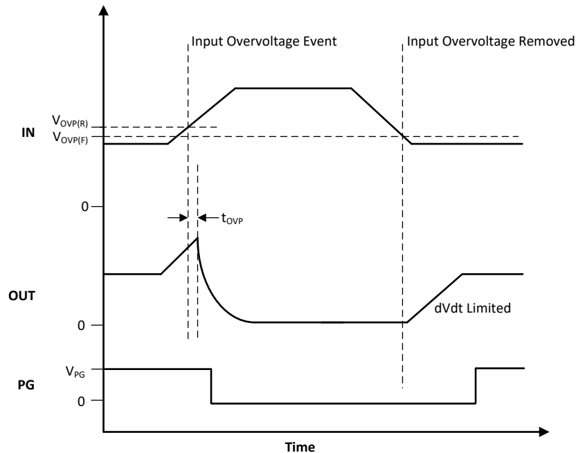
Figure 8-2. Overtolerance Response
