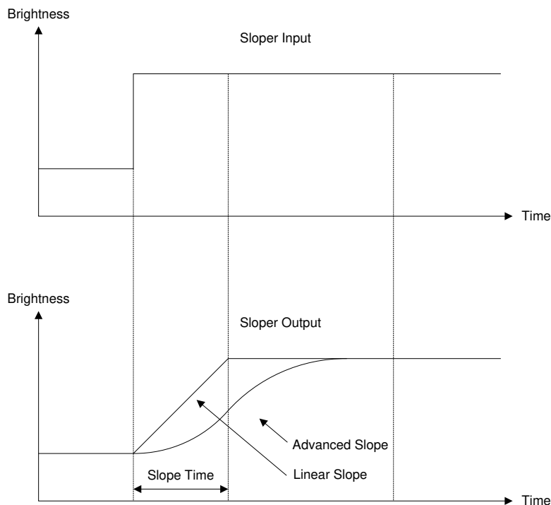
Figure 6-13. Brightness Sloper
