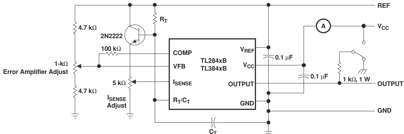
Figure 7-6. Open-Loop Laboratory Test Fixture
