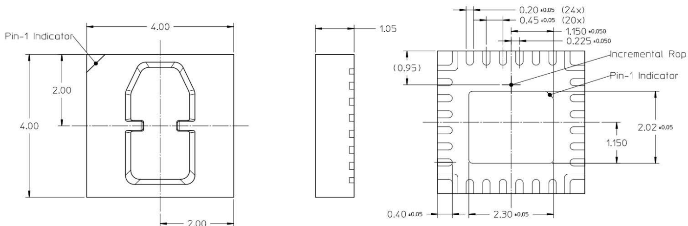
Figure 11: Package Outline Drawing
