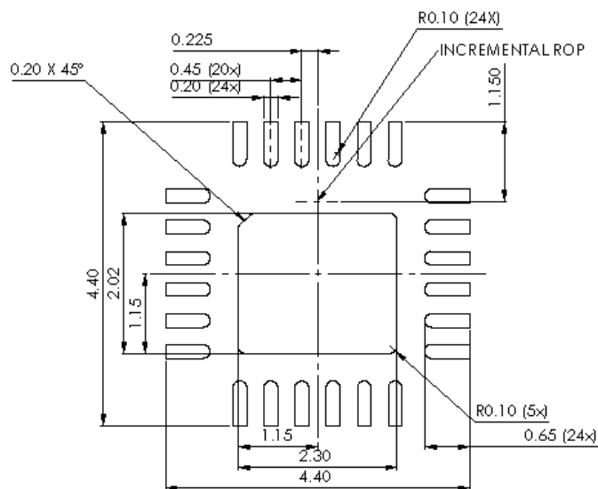
Figure 12: Recommended Land Pattern
