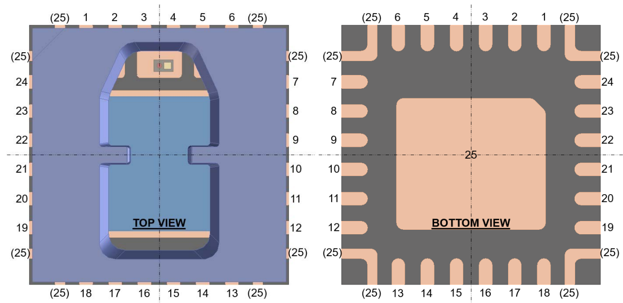
Figure 4: Encoder Pinout
