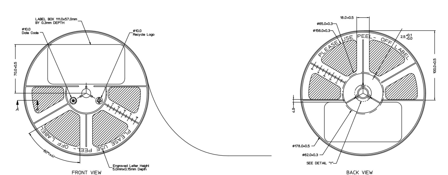
Figure 17: Reel Dimensions
