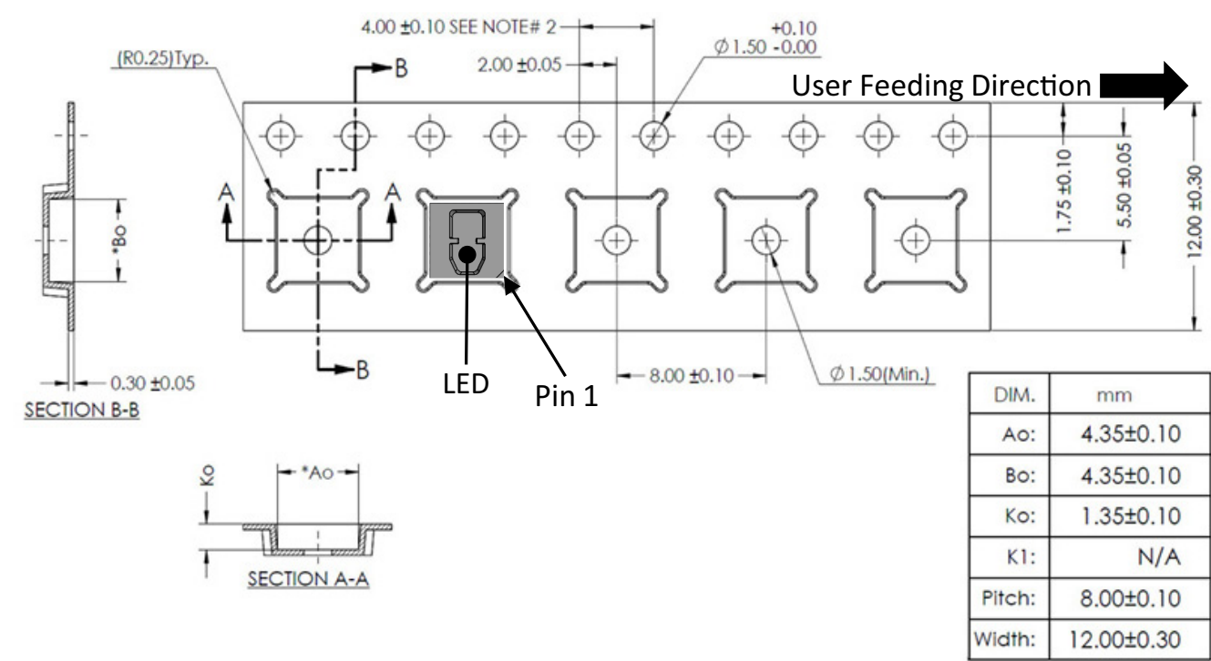
Figure 16: Tape and Reel Information
