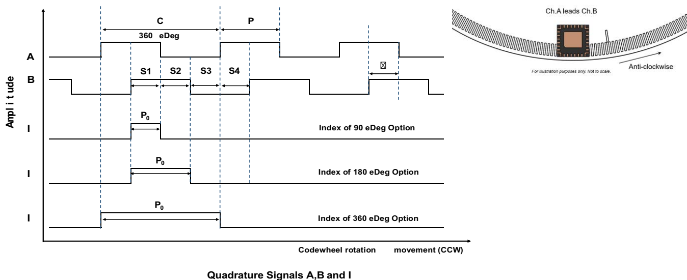
Figure 3: Digital Output Option
