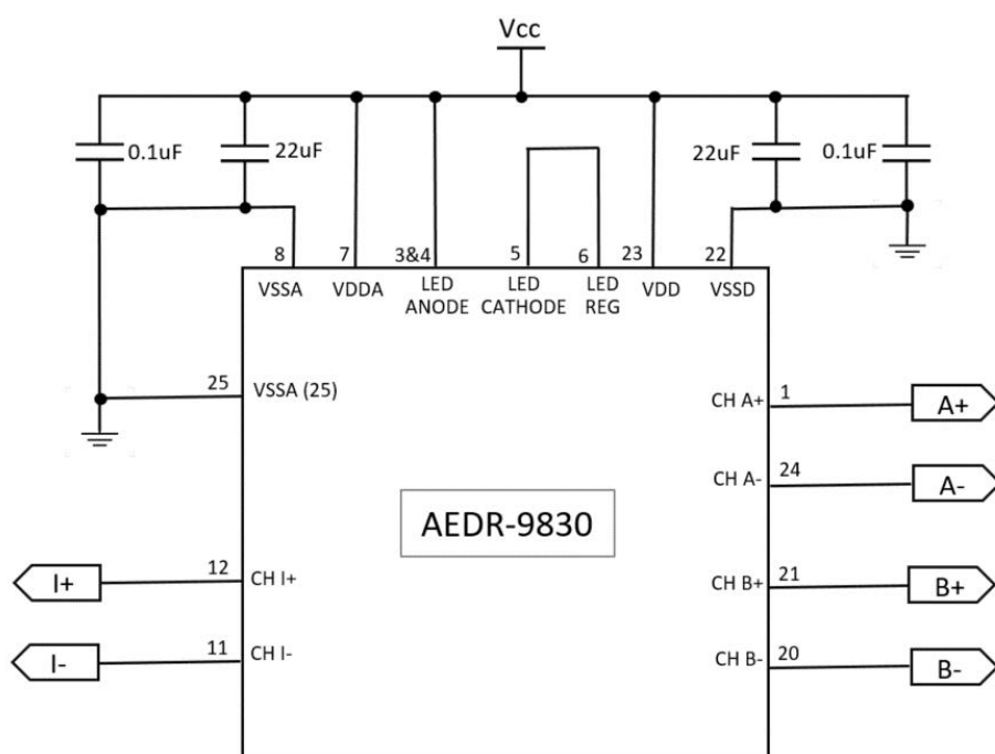
Figure 6: Connection Diagram
