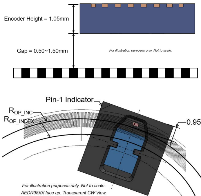
Figure 13: Encoder Placement Orientation
