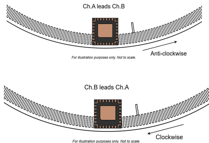
Figure 14: Channel Leads
