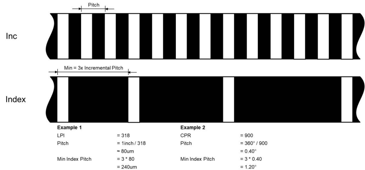
Figure 10: Multiple Index Pulse Design
