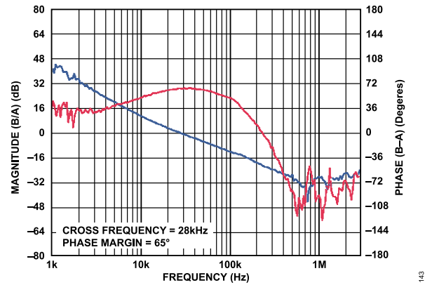
Figure 43. ADP2303 Bode Plot, V_{OUT} = 5\text{ V} , V_{IN} = 12\text{ V} , L = 4.7\text{ }\mu\text{H} , C_{OUT} = 47\text{ }\mu\text{F}
