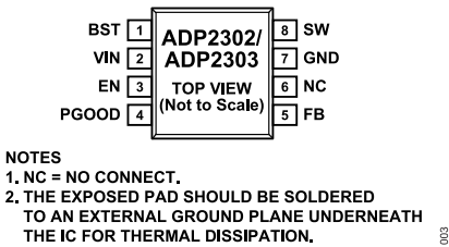
Figure 3. Pin Configuration (Top View)
