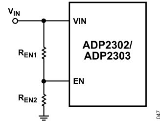
Figure 49. Precision Enable Used as a Programmable UVLO
