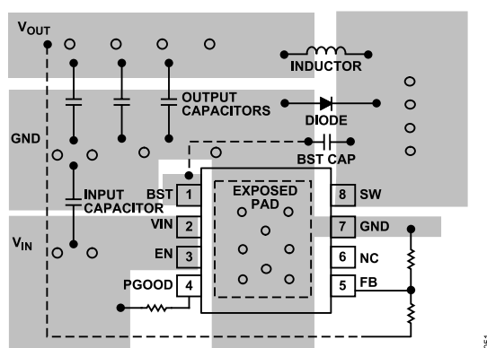
Figure 53. Recommended Layout for ADP2302/ADP2303
