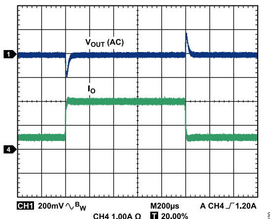
Figure 30. ADP2302 Load Transient, 0.5 A to 2.0 A, V_{OUT} = 5.0\text{ V} , V_{IN} = 12\text{ V} , L = 6.8\text{ μH} , C_{OUT} = 2 \times 22\text{ μF}
