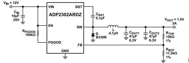
Figure 54. ADP2302 Typical Application, V_{IN} = 12\text{ V} , V_{OUT} = 1.5\text{ V} , 2\text{ A}
