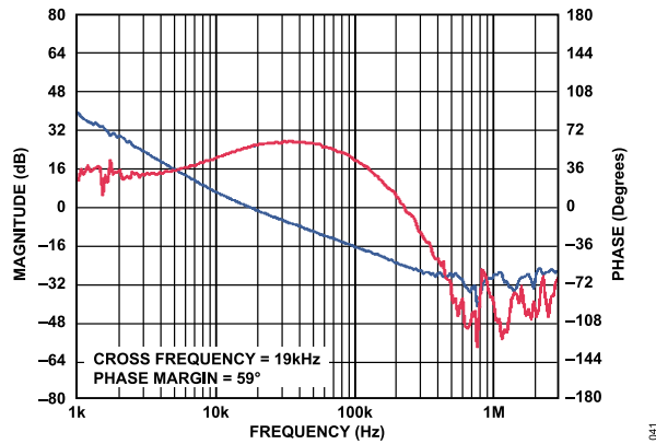
Figure 41. ADP2303 Bode Plot, V_{OUT} = 3.3\text{ V} , V_{IN} = 12\text{ V} , L = 4.7\text{ }\mu\text{H} , C_{OUT} = 2 \times 47\text{ }\mu\text{F}
