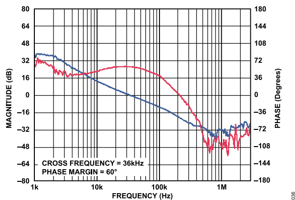
Figure 36. ADP2302 Bode Plot, V_{OUT} = 2.5\text{ V} , V_{IN} = 12\text{ V} , L = 4.7\text{ }\mu\text{H} , C_{OUT} = 3 \times 22\text{ }\mu\text{F}
