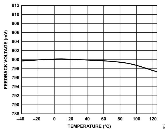
Figure 19. 0.8 V Feedback Voltage vs. Temperature
