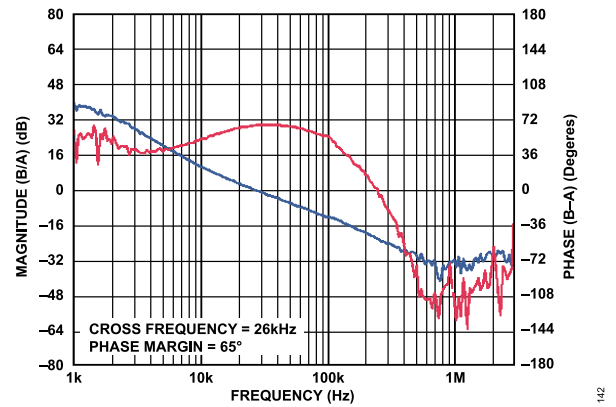
Figure 42. ADP2303 Bode Plot, V_{OUT} = 2.5\text{ V} , V_{IN} = 12\text{ V} , L = 3.3\text{ }\mu\text{H} , C_{OUT} = 2 \times 47\text{ }\mu\text{F}
