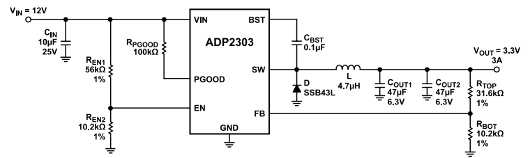
Figure 51. Schematic for the Design Example
