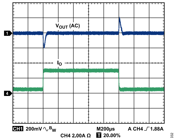
Figure 32. ADP2303 Load Transient, 0.5 A to 3.0 A, V_{OUT} = 3.3\text{ V} , V_{IN} = 12\text{ V} , L = 4.7\text{ μH} , C_{OUT} = 2 \times 47\text{ μF}
