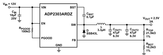
Figure 61. ADP2303 Typical Application, V_{IN} = 12\text{ V} , V_{OUT} = 2.5\text{ V} , 3\text{ A}
