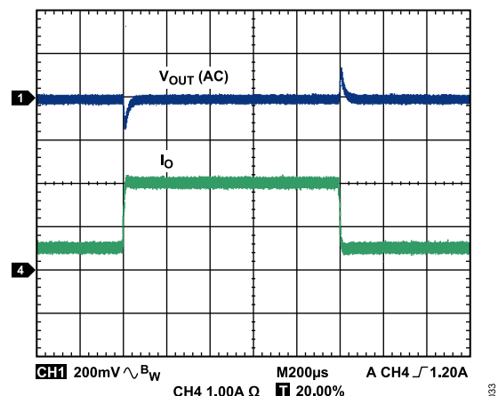
Figure 33. ADP2302 Load Transient, 0.5 A to 2.0 A, V_{OUT} = 3.3\text{ V} , V_{IN} = 12\text{ V} , L = 6.8\text{ μH} , C_{OUT} = 2 \times 22\text{ μF}
