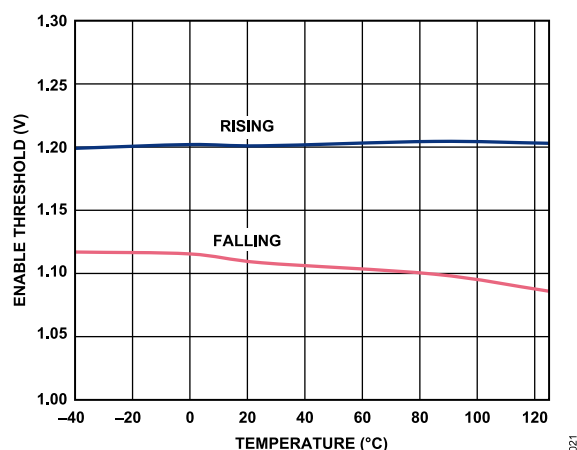
Figure 21. Enable Threshold vs. Temperature
