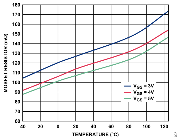
Figure 23. MOSFET R_{DS(on)} vs. Temperature (Pin-to-Pin Measurement)
