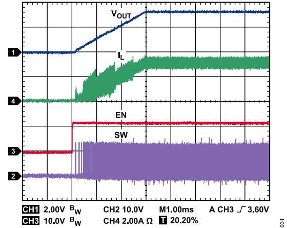
Figure 31. Soft Start with Full Load, V_{OUT} = 3.3\text{ V} , V_{IN} = 12\text{ V}
