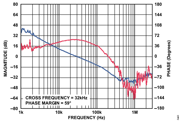
Figure 40. ADP2302 Bode Plot, V_{OUT} = 5\text{ V} , V_{IN} = 12\text{ V} , L = 6.8\text{ }\mu\text{H} , C_{OUT} = 2 \times 22\text{ }\mu\text{F}
