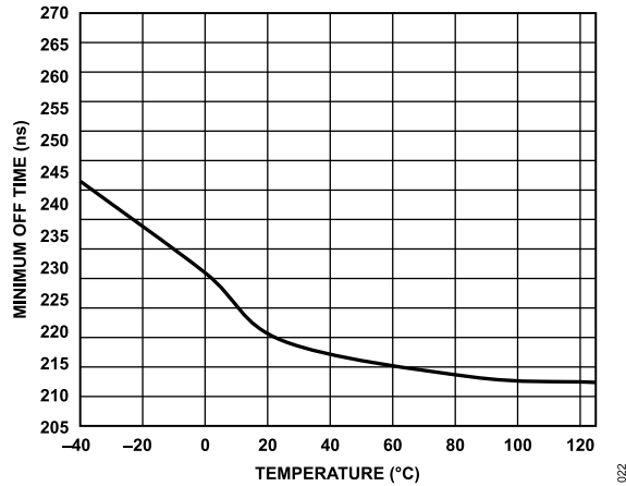
Figure 22. Minimum Off Time vs. Temperature
