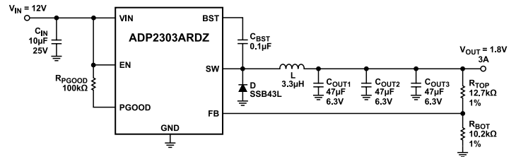
Figure 60. ADP2303 Typical Application, V_{IN} = 12\text{ V} , V_{OUT} = 1.8\text{ V} , 3\text{ A}
