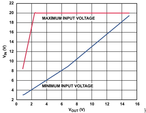
Figure 47. Voltage Conversion Limitations
