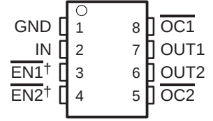
TPS2042A, TPS2052A D PACKAGE (TOP VIEW)
