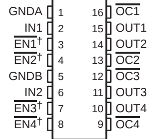
TPS2044A, TPS2054A D PACKAGE (TOP VIEW)
