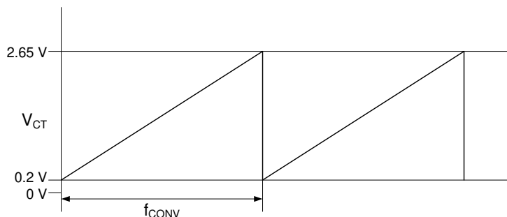
Figure 7-7. Oscillator Waveform
