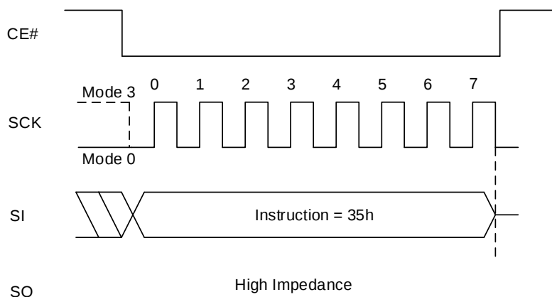
Figure 8.31 Enter Quad Peripheral Interface (QPI) Mode Sequence
