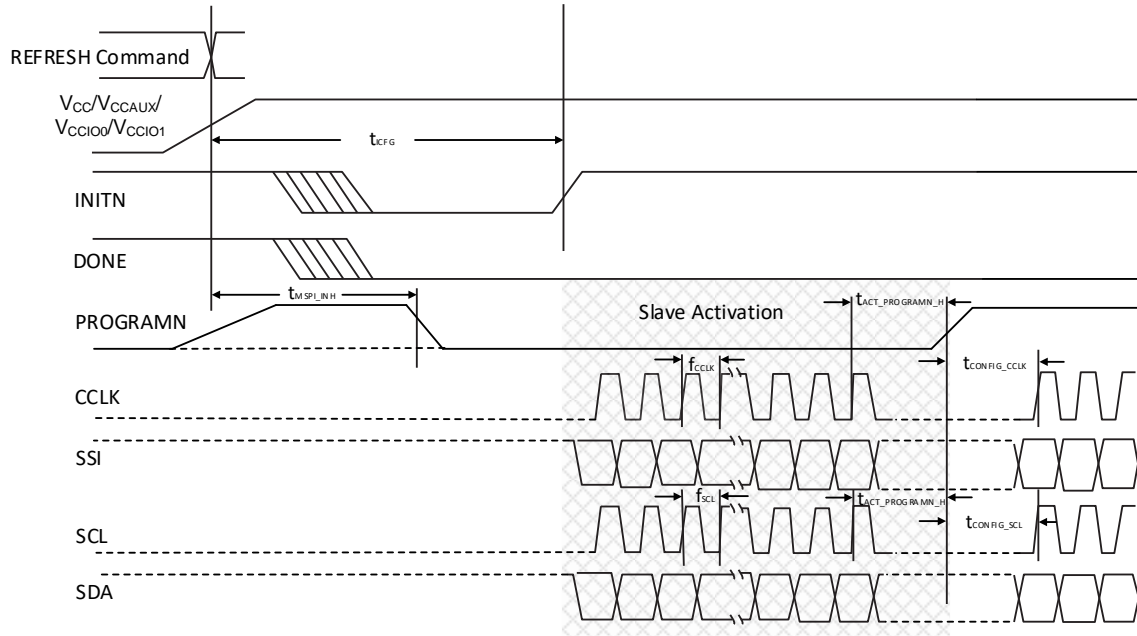
Figure 3.16. Slave SPI/i²C/I³C POR/REFRESH Timing
