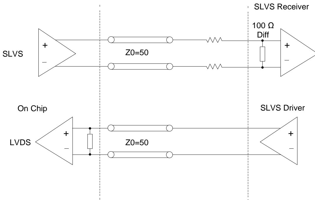
Figure 3.5. SLVS Interface
