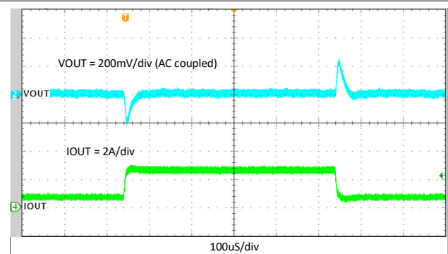
Figure 8-18. Load Transient Response, 0.5 to 2.5\text{ A} , Slew Rate = 0.8\text{ A}/\mu\text{s}
