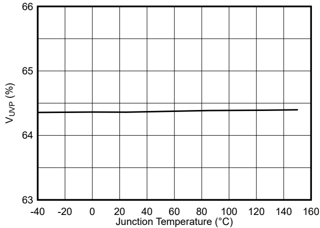
Figure 6-13. UVP Threshold vs Junction Temperature
