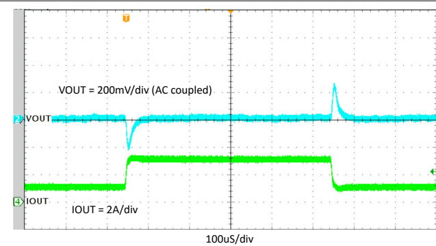
Figure 8-19. Load Transient Response, 1 to 3\text{ A} , Slew Rate = 0.8\text{ A}/\mu\text{s}
