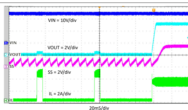
Figure 8-21. V OUT Hard Short Recovery
