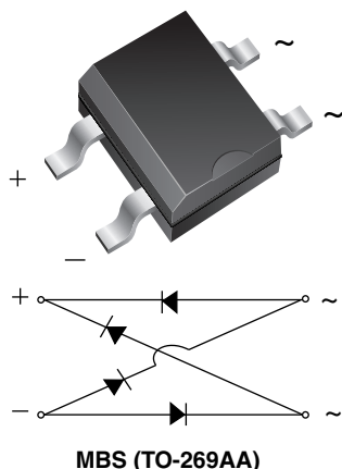
MBS (TO-269AA)
