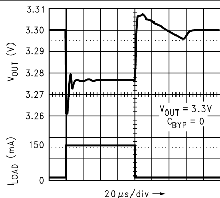
Figure 7-3. Load Transient Response for Legacy Chip
