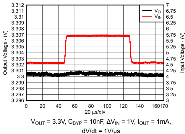
Figure 5-48. Line Transient Response (New Chip)
