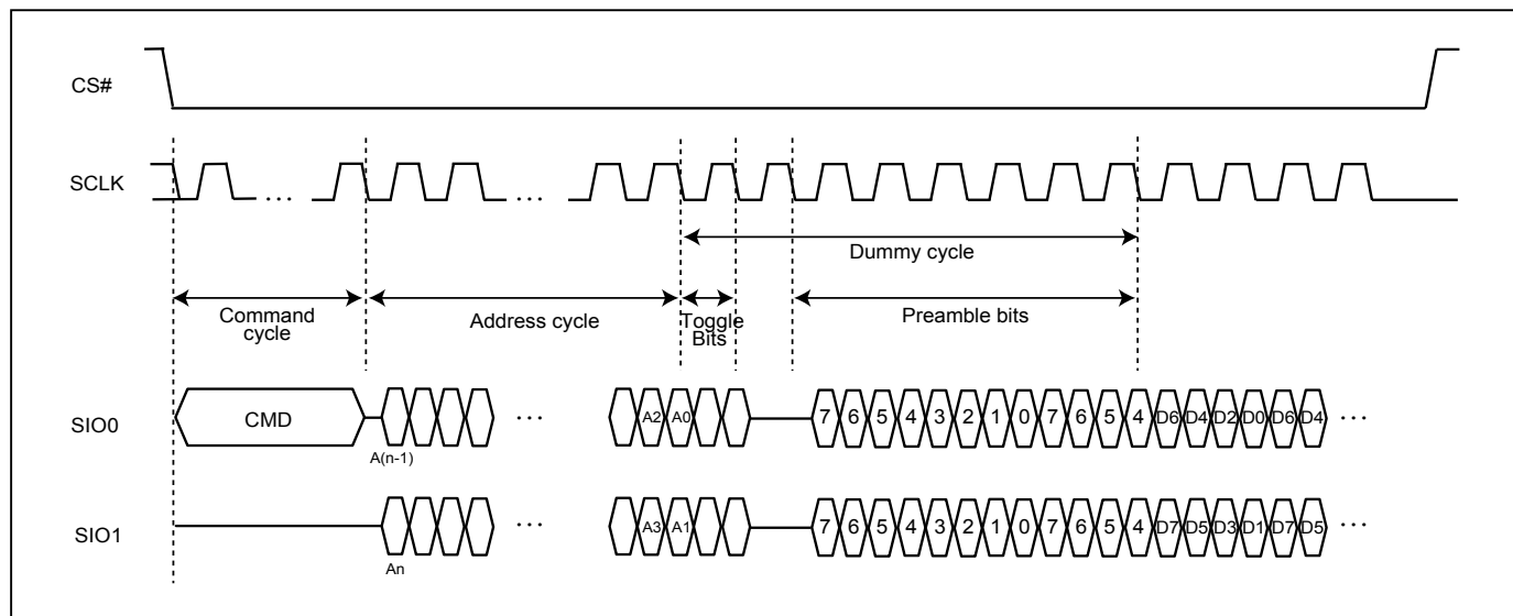
Figure 54. DTR2IO (8DC)
