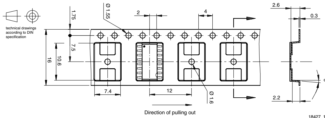
Fig. 16 - 2000 pcs/reel
