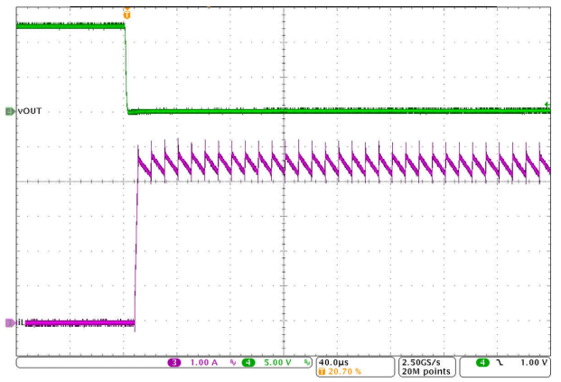
Figure 8-7. Short Circuit Applied
