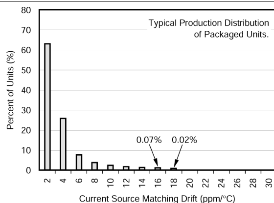
Figure 5-14. Current Source Matching Drift Production Distribution
