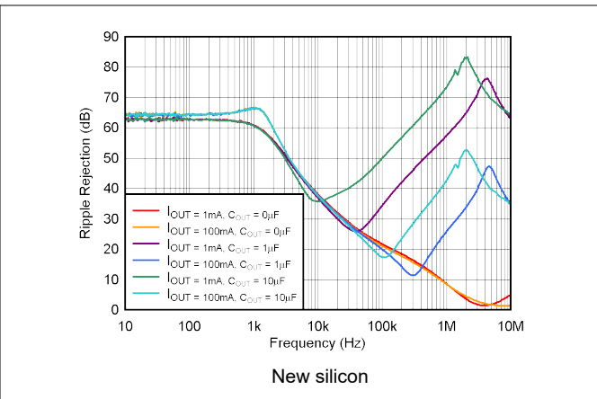
Figure 7-4. PSRR (Ripple Rejection) vs Frequency
