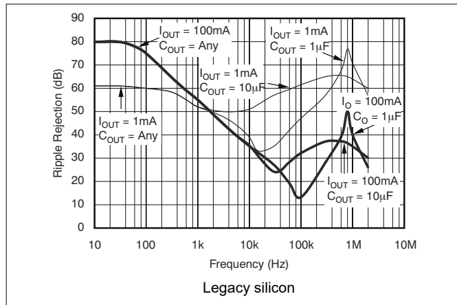
Figure 7-3. PSRR (Ripple Rejection) vs Frequency
