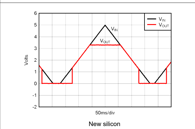
Figure 7-8. TPS73701, V_{OUT} = 3.3\text{-V} Power-Up and Power-Down
