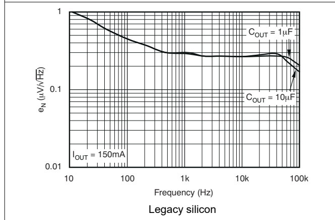
Figure 7-5. Noise Spectral Density
