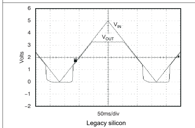
Figure 7-7. TPS73701, V_{OUT} = 3.3\text{-V} Power-Up and Power-Down
