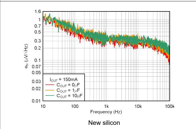
Figure 7-6. Noise Spectral Density
