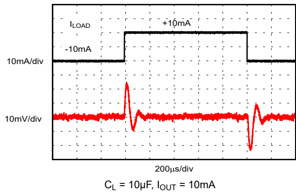
Figure 6-20. Load Transient
