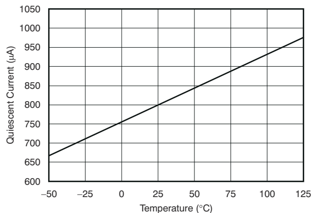
Figure 6-9. Quiescent Current vs Temperature
