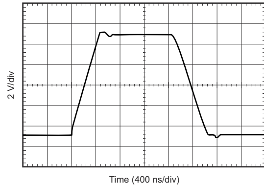
Figure 6-30. Large-Signal Step Response
