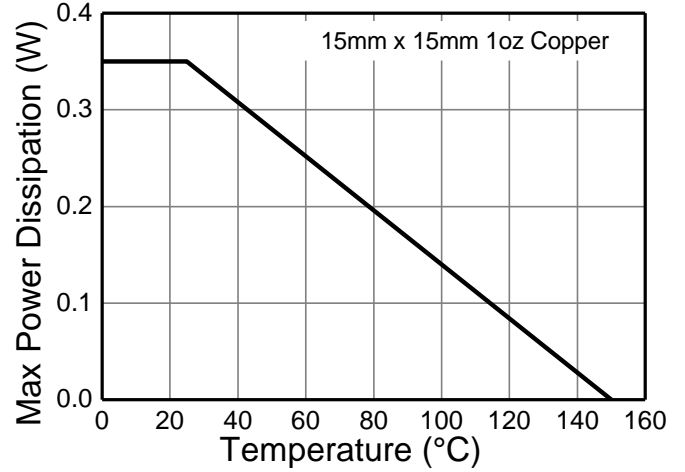
Figure 2. Derating Curve
