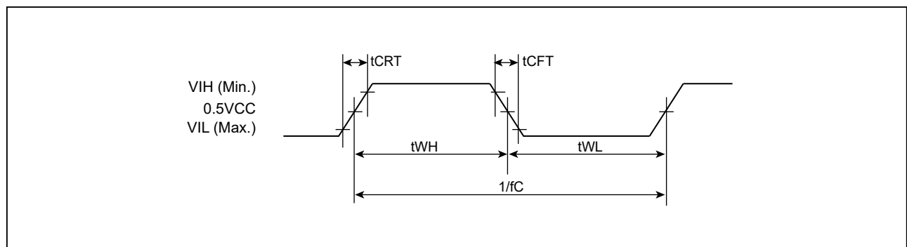
Figure 44. SCLK TIMING DEFINITION
