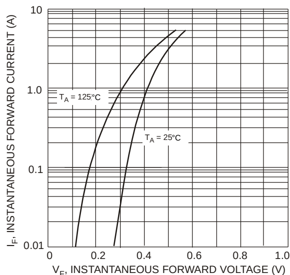
Figure 2 Typical Forward Characteristics – B350BQ/ B360BQ
