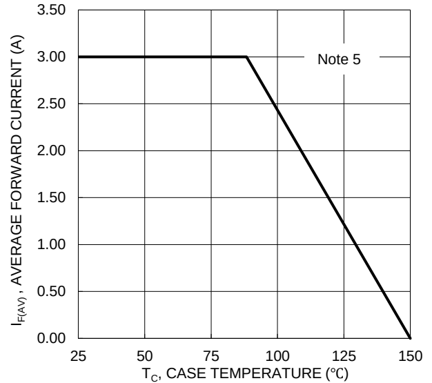
Figure 6 Forward Current Derating Curve
