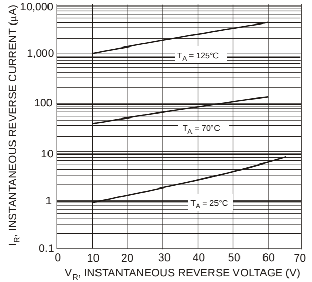
Figure 4 Typical Reverse Characteristics – B350BO/B360BO
