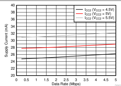
V_{\text{CC1}} = 5\text{V} , Temp = 25°C, R_L = 60 \Omega , C_{L(\text{RXD})} = 15\text{pF} Figure 6-4. Side 2 Supply Current vs Datarate
