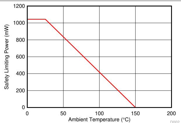
Figure 6-2. Thermal Derating Curve for Limiting Power per VDE for 8-D Package
