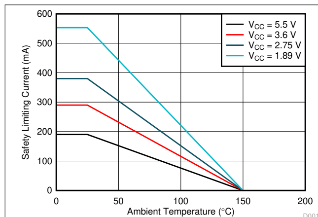
Figure 6-1. Thermal Derating Curve for Limiting Current per VDE for 8-D Package
