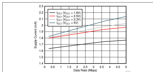
V_{\text{CC2}} = 5\text{V} , Temp = 25°C, R_L = 60 \Omega , C_{L(\text{RXD})} = 15\text{pF} Figure 6-3. Side 1 Supply Current vs Datarate
