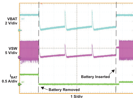
Figure 5. VBUS = 5 V, VBAT = 3.4V, I_{in\_limit} = 500\text{ mA} (32s Mode)
