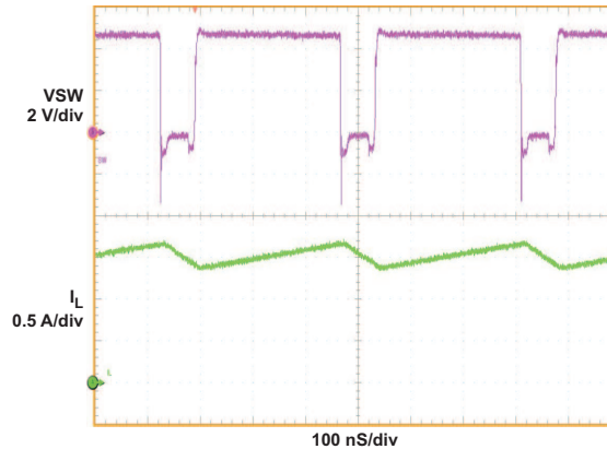
Figure 6. VBUS = 5 V, VBAT = 2.6 V, V_{reg} = 4.2\text{ V} , I_{chg} = 1550\text{ mA}
