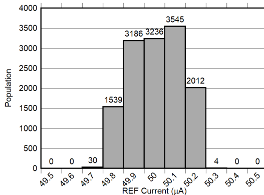
Figure 6-90. I_{REF} Distribution
