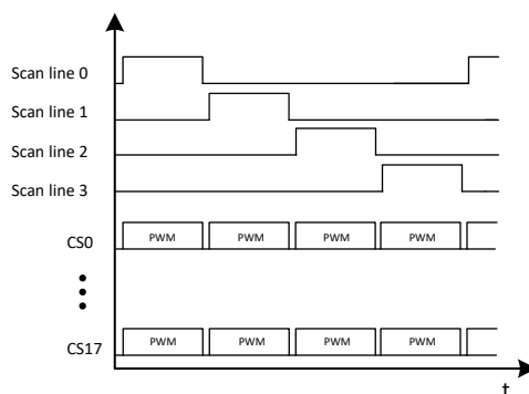
Figure 8-2. Time-Multiplexing Matrix Timing Sequence
