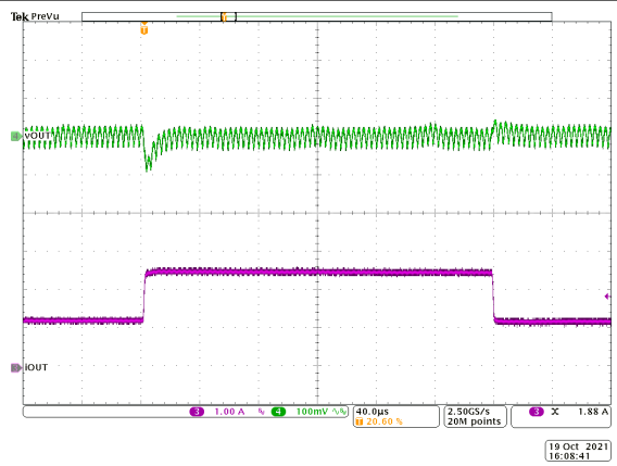
Figure 9-5. Load Step Response
